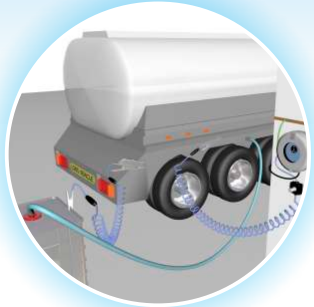
Example of grounding truck bonded to IBC
